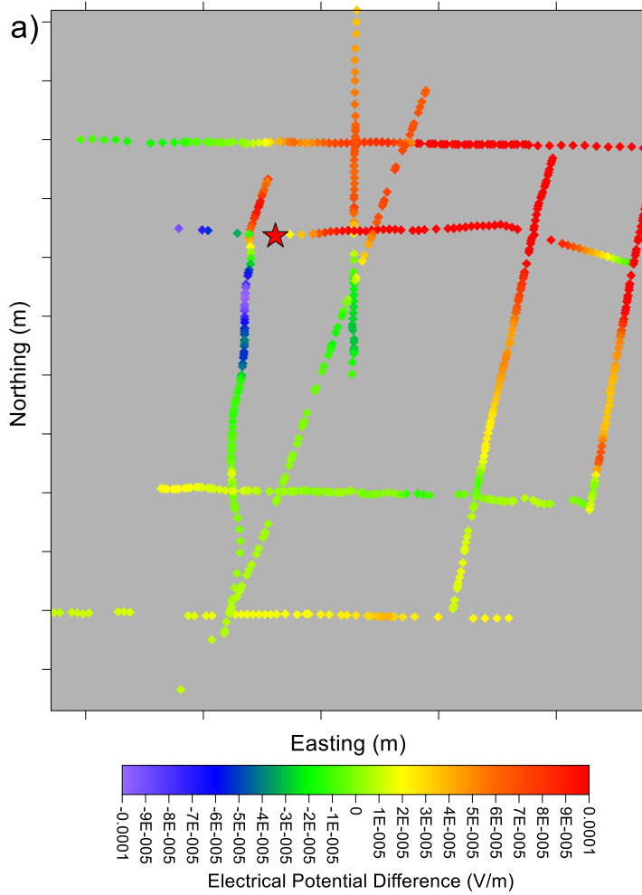
Figure 7: Raw potential differences. For typical MALM surveys this data would be used directly to interpret the limits of the subsurface conductive body. The atypical survey geometry made the usual interpretation for this dataset difficult without further processing
