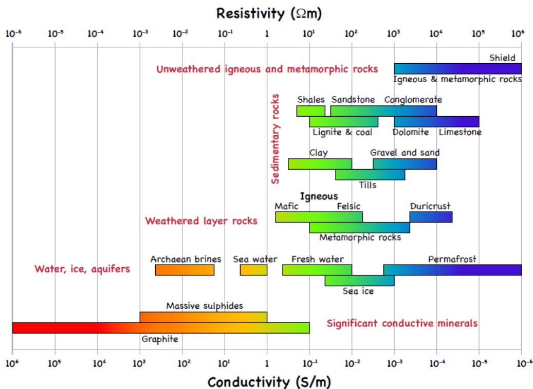
Figure 1: Typical ranges of electrical resistivities for common subsurface materials (from Yeomans, 2011). For this study, it is important to note that salt water is orders of magnitude less resistive than the host formation sands.
