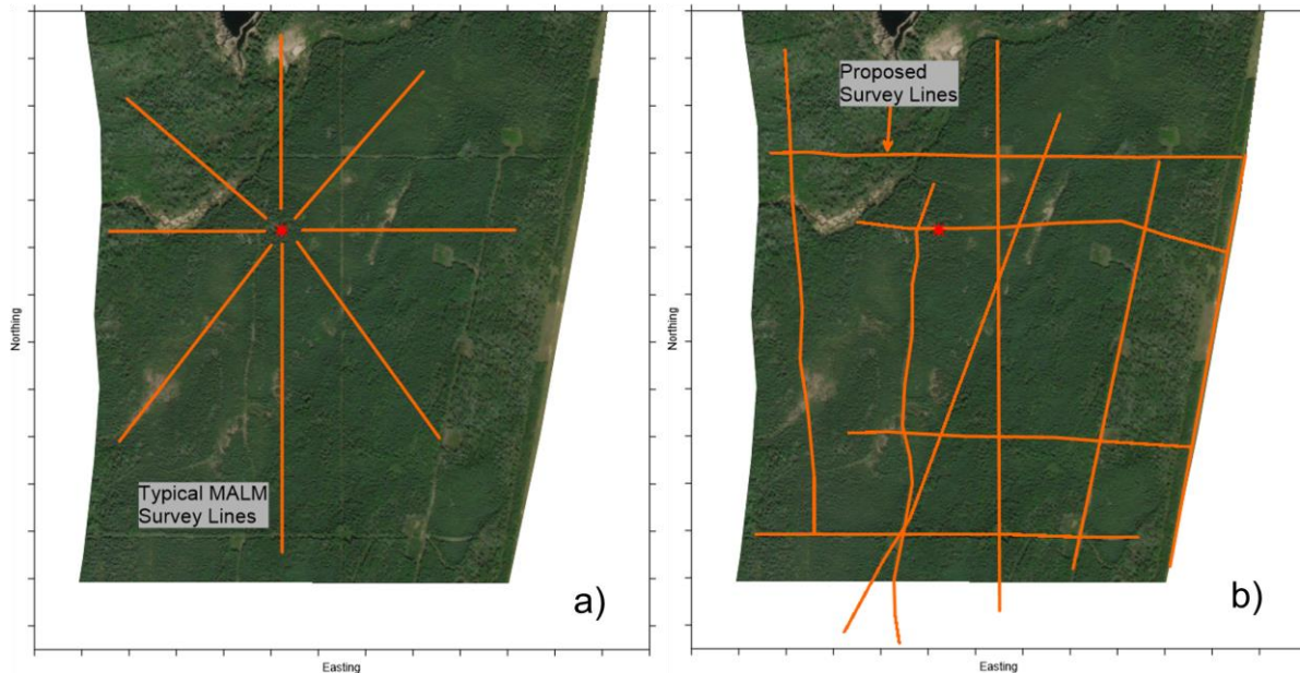
Figure 5: Illustration of a) typical MALM acquisition setup and b) the survey lines that were available for this survey. The well that encountered the high-TDS aquifer is marked in red.
