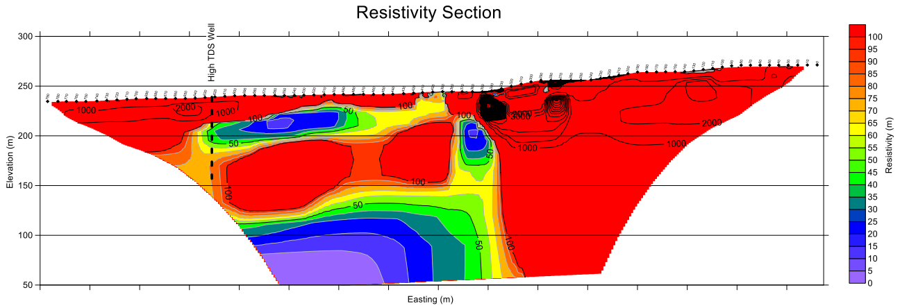
Figure 6: Results from the ERT survey. These results show that there is a conductive unit to the east of the well that noted the high-TDS water sample.
