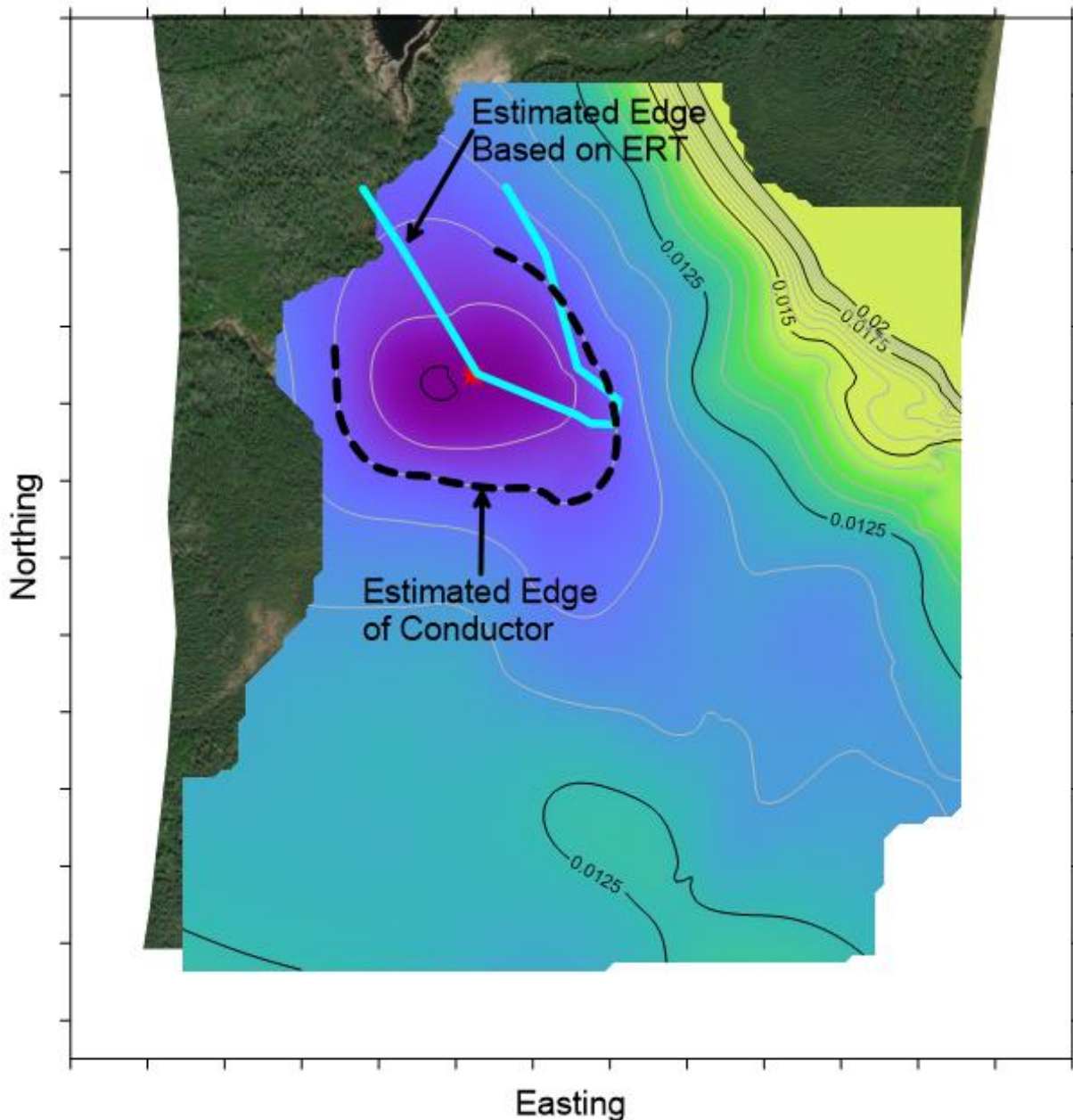
Figure 8: Processed potential difference surface. The limit of the conductive aquifer based on the MALM is indicated by the dashed black line. The limit of the conductive aquifer based on the ERT is indicated by the cyan line. The difference between the two limits is likely due to the limitations of the ERT when the aquifer becomes very thin.
